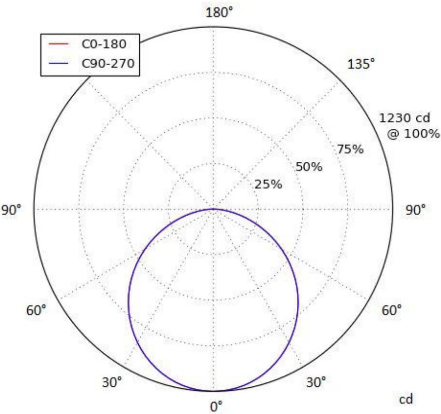
Figure. Polar curve of the angular Luminous Intesity distribution at two perpendicular C planes and at C plane with maximum Luminous Intesity.
